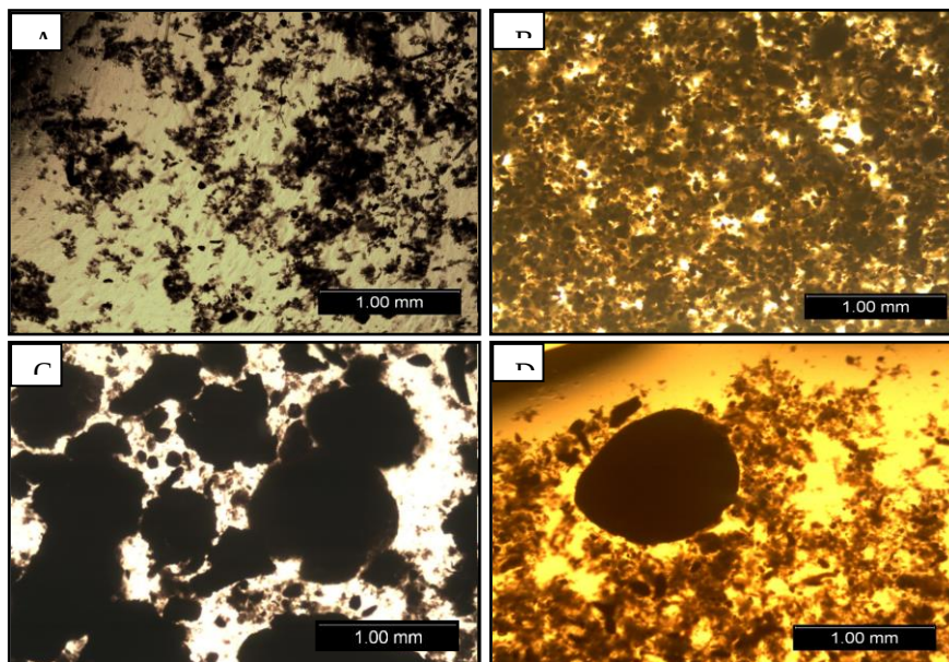
Figure 4. The morphological variation of granules captured using the PAX-IT™ during the experimental period (magnification = 40x). (A) Raw sludge; (B) after 28 days; (C) after 75 days and (D) after 90 days.
