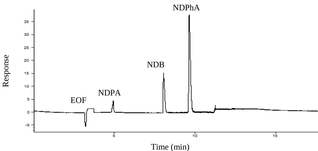
Figure 8. Electropherogram of a nitrosamine standard mixture at 200 µg/mL, after the optimization steps Separation conditions: 40 mM SDS in 10 mM phosphate buffer (pH 8); capillary 64.5 cm × 50 µm I.D (effective length, 56 cm); applied voltage 29 kV; temperature, 25 °C; Injection electrokinetic, 5 kV/9 sec.
