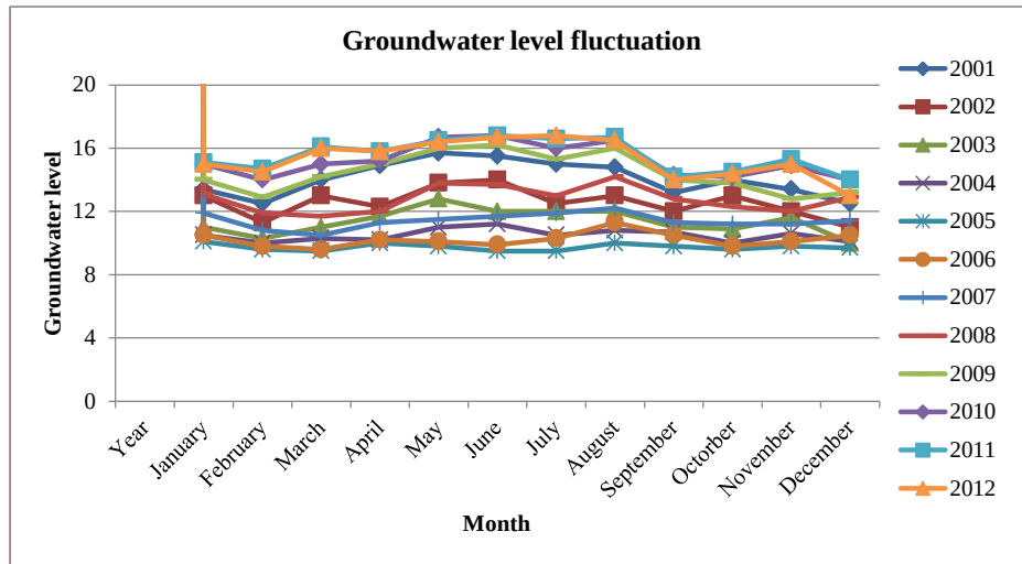
Figure 9. Water table fluctuations of Terengganu, Malaysia during 2001 to 2012
