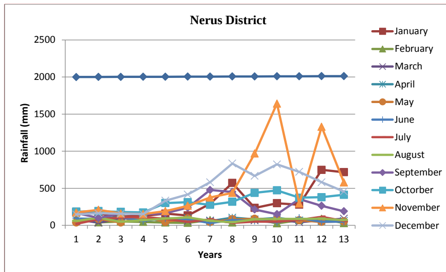
Figure 2. Monthly rainfall variations at Nerus District from 2001 to 2013
