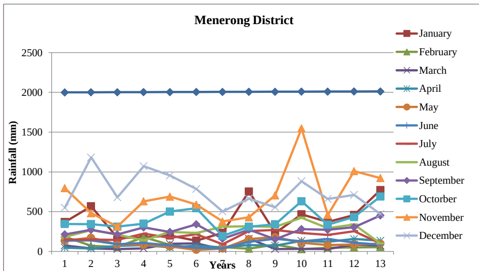
Figure 6. Monthly rainfall variations at Menerong District from 2001 to 2013
