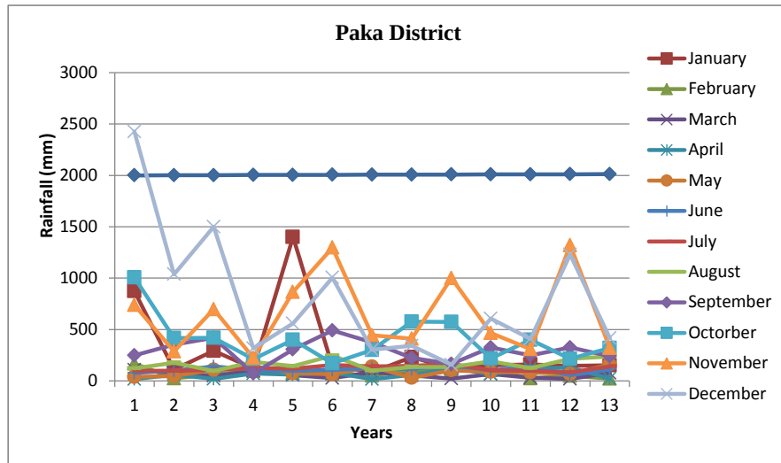
Figure 3. Monthly rainfall variations at Paka District from 2001 to 2013
