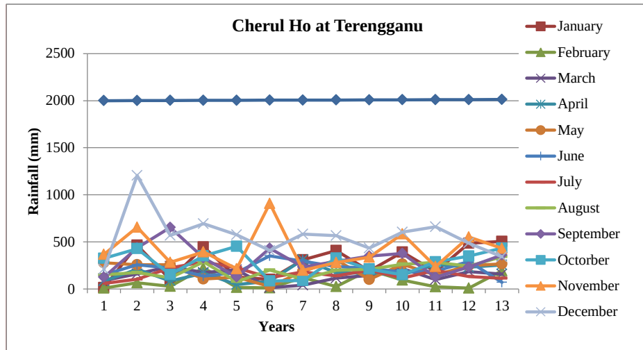
Figure 7. Monthly rainfall variations at Cherul District from 2001 to 2013
