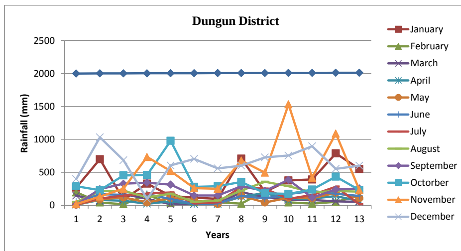
Figure 4. Monthly rainfall variations at Dungun District from 2001 to 2013
