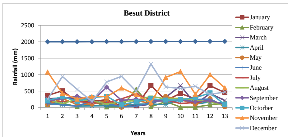
Figure 8. Monthly rainfall variations at Besut District from 2001 to 2013
