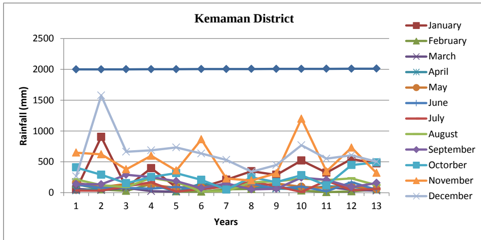
Figure 5. Monthly rainfall variations at Kemaman District from 2001 to 2013
