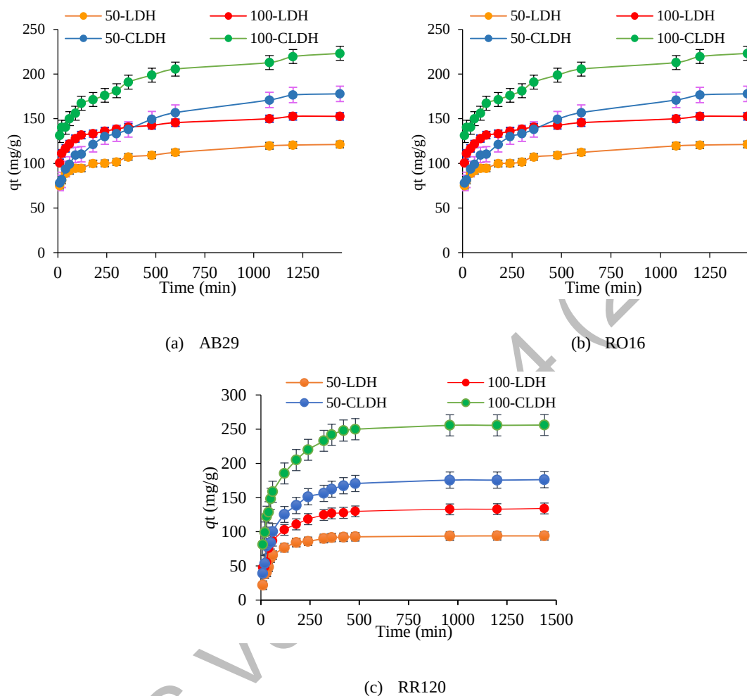
Figure 6. Effect of contact time and initial dye concentrations on adsorption capacity in adsorption by LDH and CLDH on anionic dyes (a)AB29, (b) RO16 and (c) RR120
