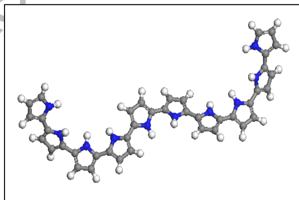
The optimized structure of PPy with 10 monomers of pyrrole Figure 4. The optimize structure Ppy consists of 10 monomers of pyrrole
