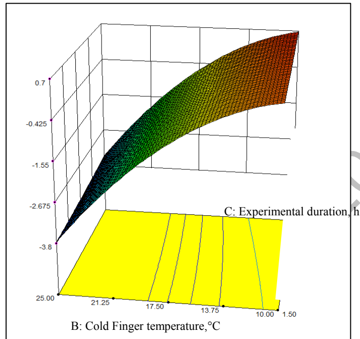
Figure 3. The comparison of predicted and experimental values of wax deposit amount using CCD
