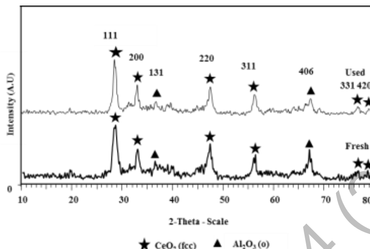
Figure 8. XRD diffractograms of fresh and used \text{Ce}/\text{Al}_2\text{O}_3 catalysts calcined at 1000 °C for 5 hours
