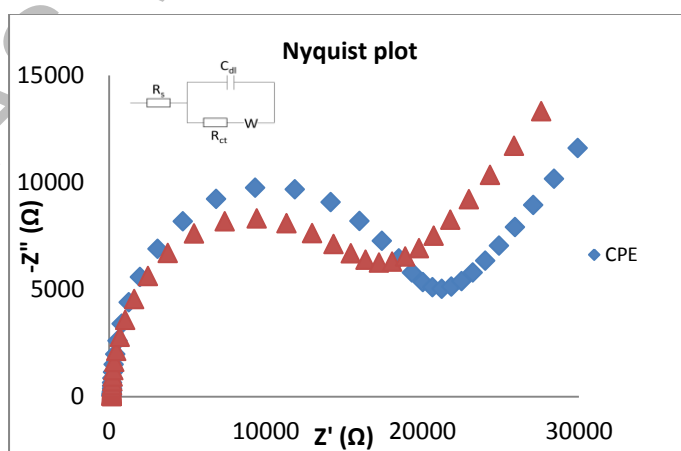
Figure 6. Nyquist plot at CPE and MCPE in of 1mM of \text{Fe}(\text{CN})_3\text{-}4\text{-}6 containing 0.1 M KCl as supporting electrolyte
