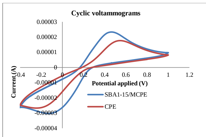
Figure 5. Cyclic voltammograms of 1mM of \text{Fe}(\text{CN})_3\text{-}4\text{-}6 containing 0.1 M KCl as supporting electrolyte at CPE and MCPE
