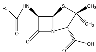
Figure 1. General structure of PENs (R = lateral amino chain)
